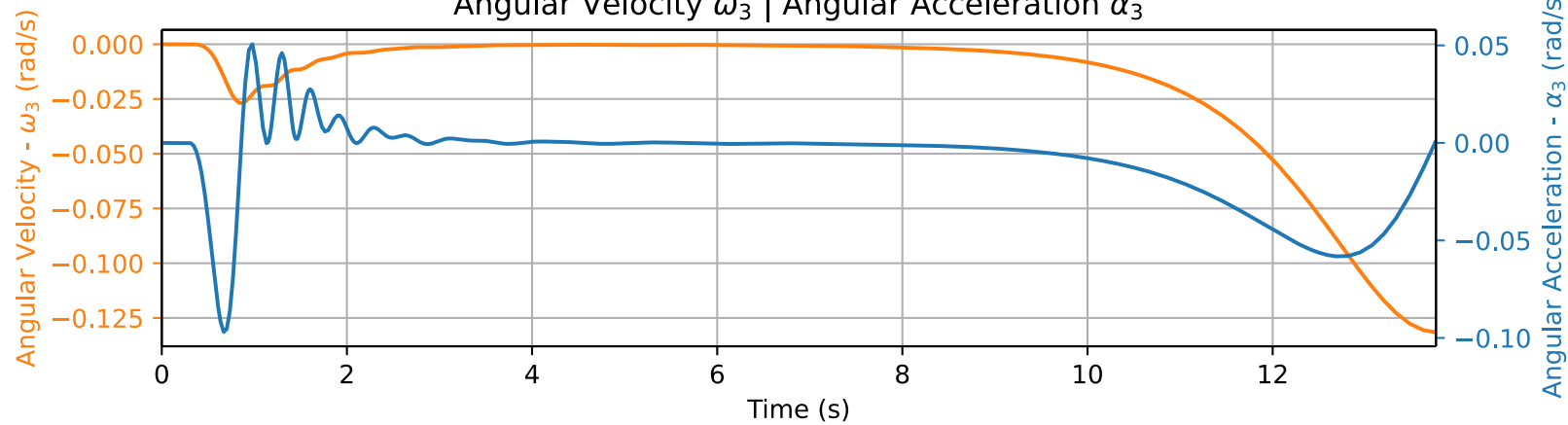
Angular Velocity \omega_3 | Angular Acceleration \alpha_3
